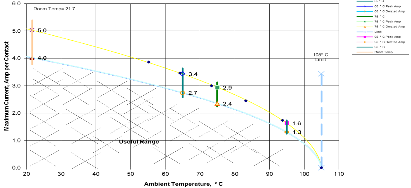
193140 (Contact Interface) 50 (All Power) Contacts in Series Part Numbers: MMSD-25-20-L-12.00-D-K-LUS / IPL1-125-01-L-D-K Current Rating per Contact (30 Deg. Rise, 20% Derated) = 2.4 Amps
