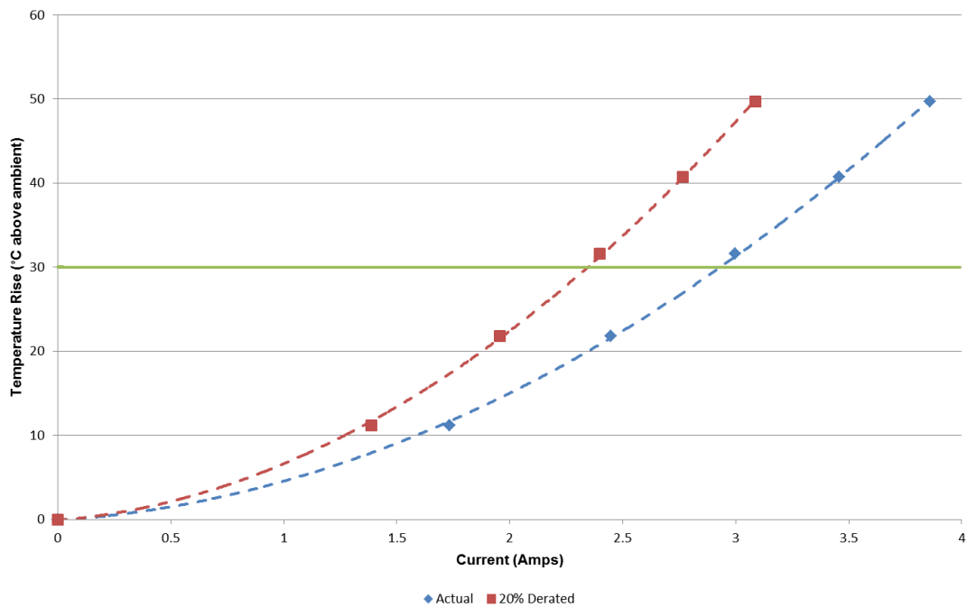
193140 (Contact Interface) 50 (All Power) Contacts in Series Part Numbers: MMSD-25-20-L-12.00-D-K-LUS / IPL1-125-01-L-D-K
