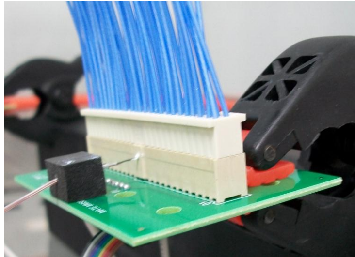
PREPARED TEST SAMPLE
