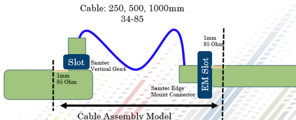
Figure 2: Diagram of the DUT
