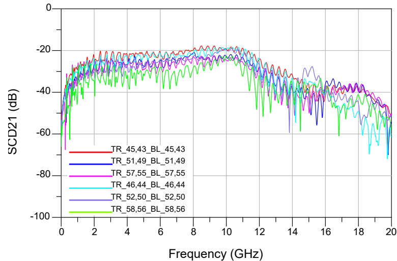
9.80 inches:Differential to Common Mode Conversion - SCD21
