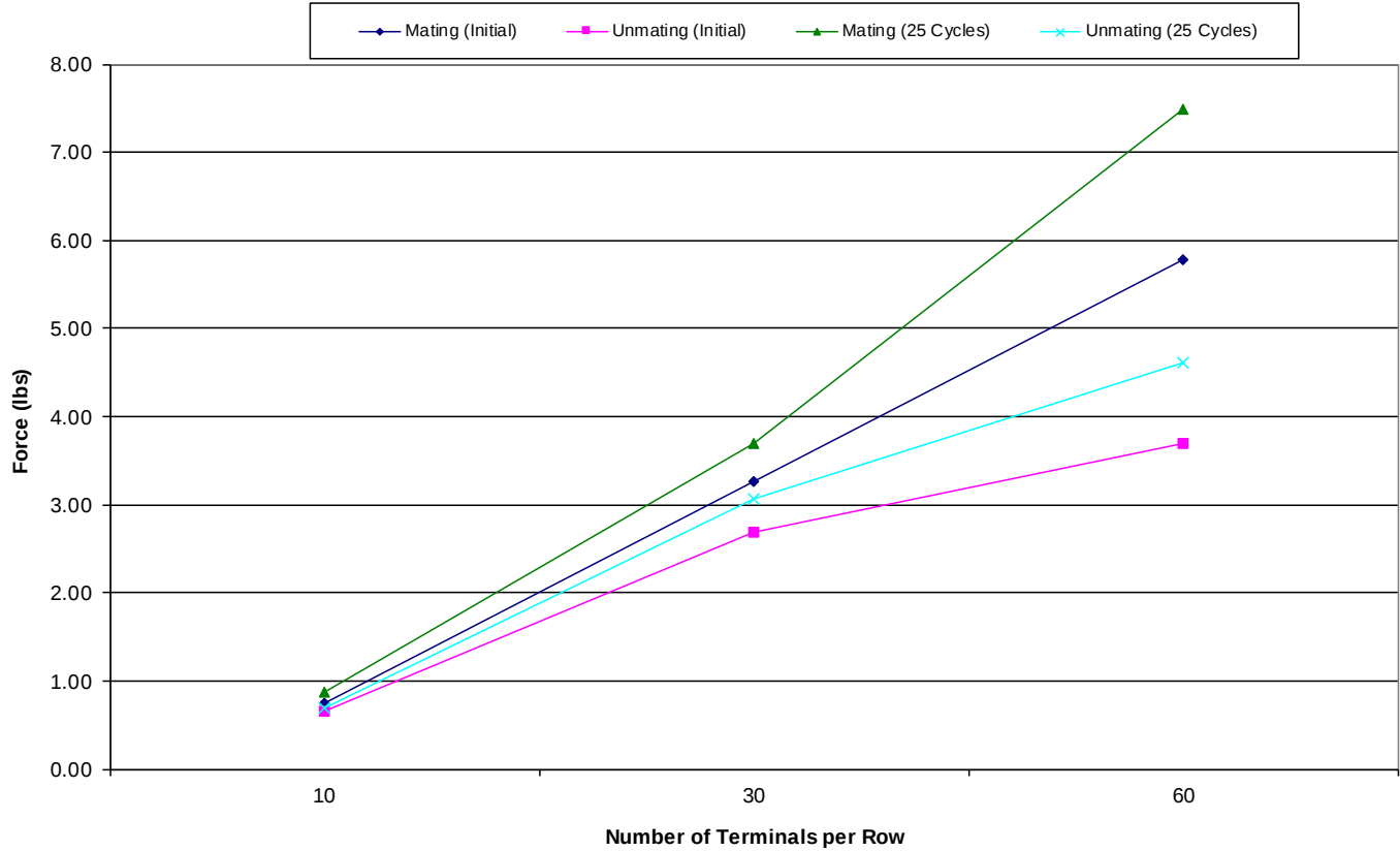
Mating/Unmating Data for 10, 30 and 60 Position ERF6/ERM6
