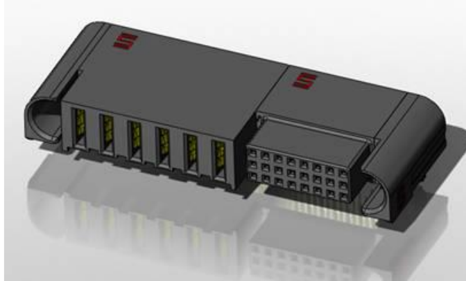
Right Angle Socket Power Assembly ET60S-00-24-06-L-RT1-GP ET60T-00-24-06-L-RT1-GP
