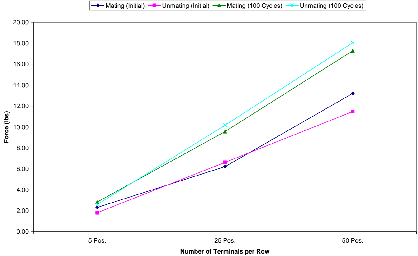
Mating/Unmating Data for 5, 25 and 50 Position SFM/FTSH
