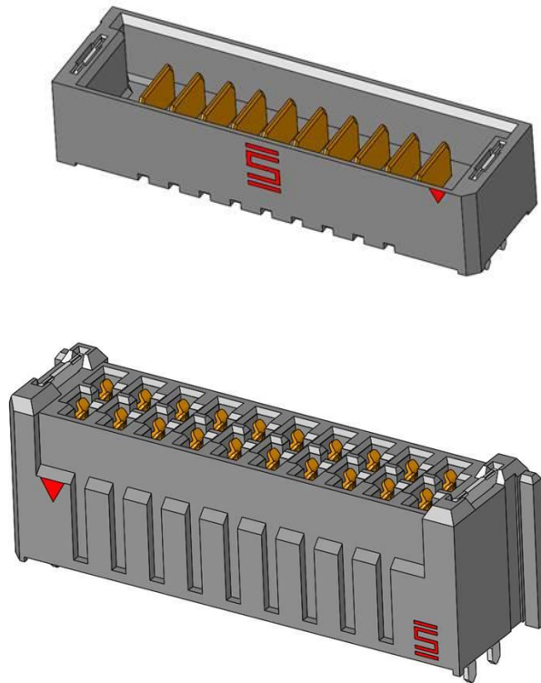
UMPT/UMPS UMPS-10-07.5-G-V-S-W-XR /UMPT-10-12.5-G-V-S-W-XR
