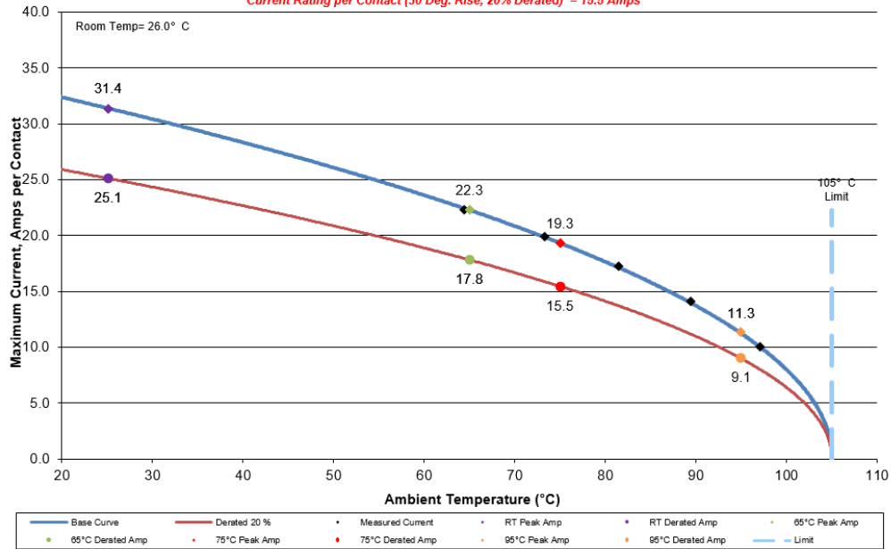
2476732 2 (1x2) Signal Pins Powered in Series Part Numbers: UMPS-10-07.5-T-V-S-W-XR/UMPT-10-12.5-T-V-S-W-XR
