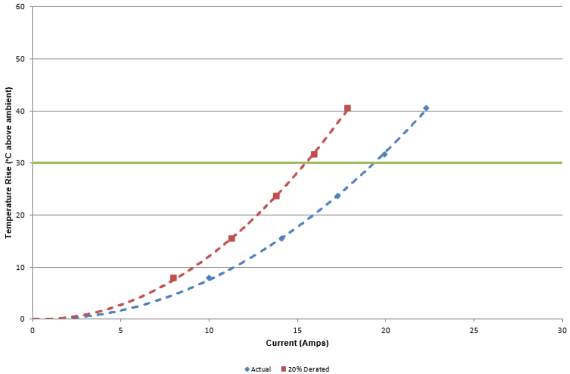
2476732 2 (1x2) Signal Pins Powered in Series Part Numbers: UMPS-10-07.5-T-V-S-W-XR/UMPT-10-12.5-T-V-S-W-XR
