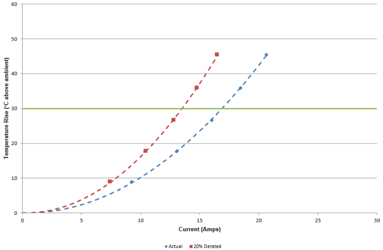
2501776 3 (1x3) Signal Pins Powered in Series Part Numbers: UMPS-10-05.5-T-V-S-W-XR /UMPT-10-06.5-T-V-S-W-XR
