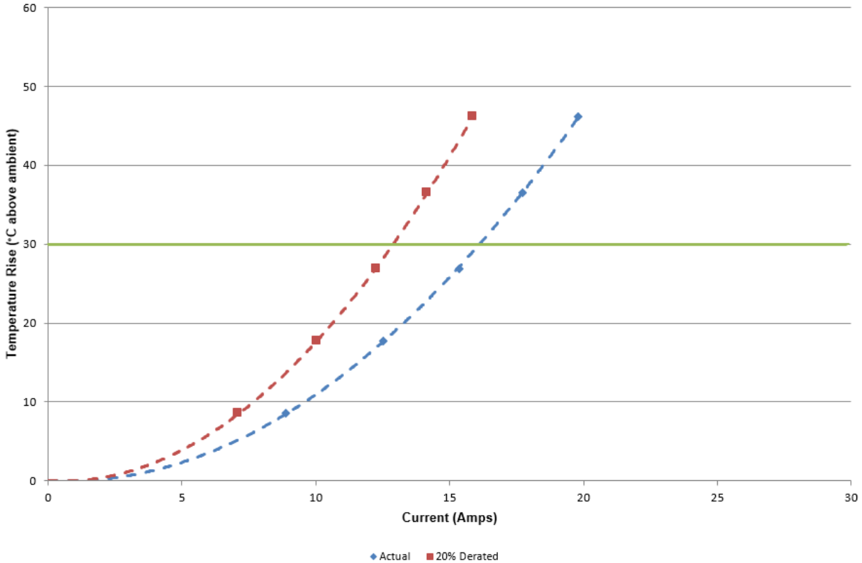
2501776 4 (1x4) Signal Pins Powered in Series Part Numbers: UMPS-10-05.5-T-V-S-W-XR /UMPT-10-06.5-T-V-S-W-XR
