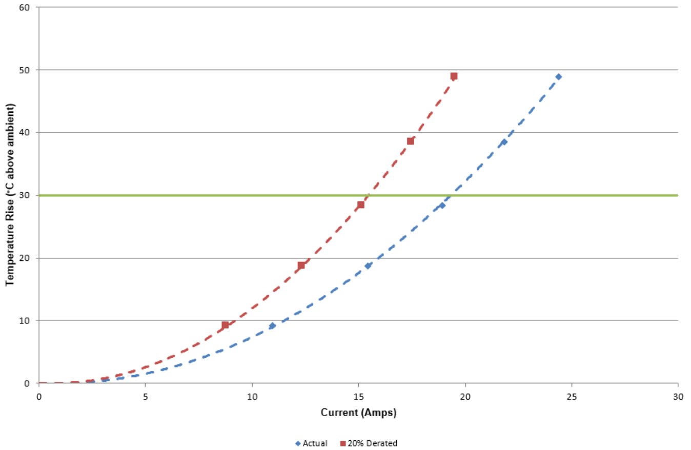
2501776 2 (1x2) Signal Pins Powered in Series Part Numbers: UMPS-10-05.5-T-V-S-W-XR /UMPT-10-06.5-T-V-S-W-XR
