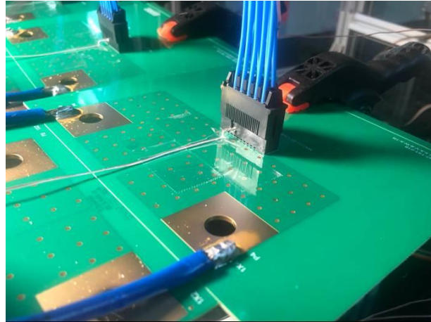
PREPARED TEST SAMPLE
