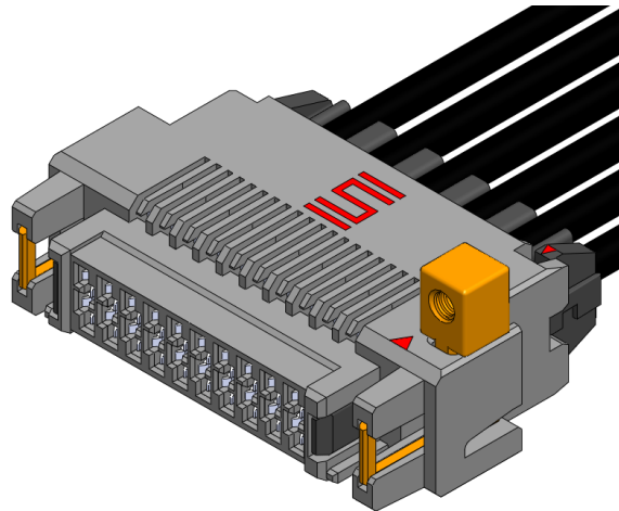
UMPE/UMPI UMPE-10-T-16-12.0/UMPI-10-T-16-12.0
