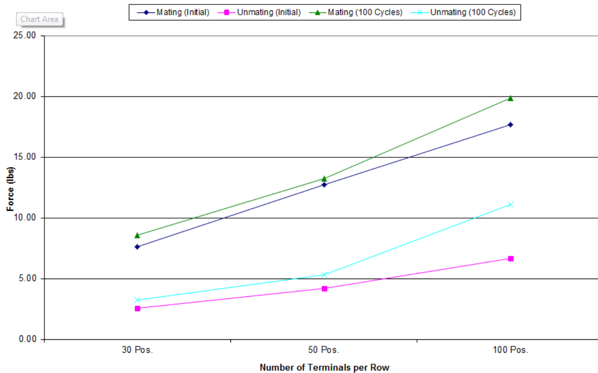
Mating/Unmating Data for 30, 50 and 100 Position MEC5/CARD
