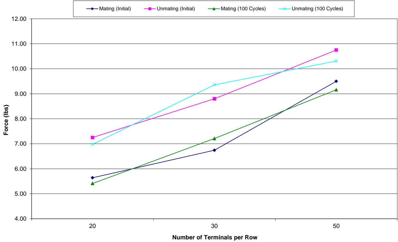
Mating/Unmating Data for 20, 30 and 50 Position LSHM/LSHM---Lubed
