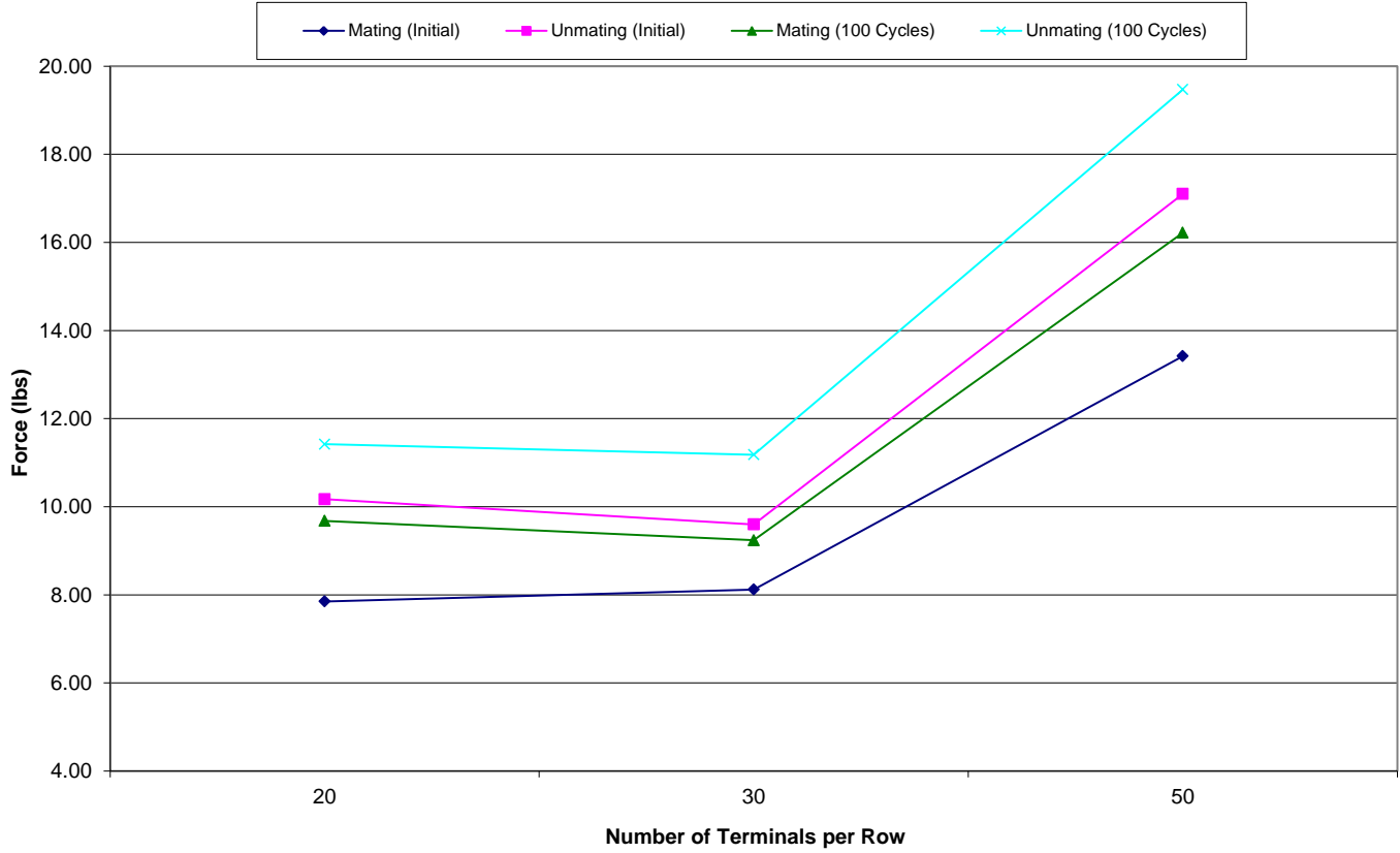
Mating/Unmating Data for 20, 30 and 50 Position LSHM/LSHM---Non Lubed
