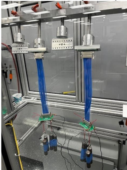
Fig. 3 (Standard setup)
