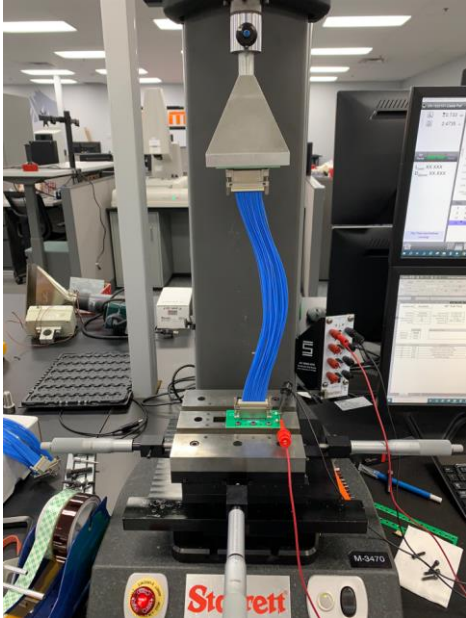
Fig. 1 0^\circ Connector pull.
