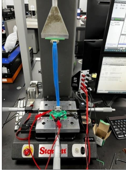
Fig. 1 0^\circ Connector pull
