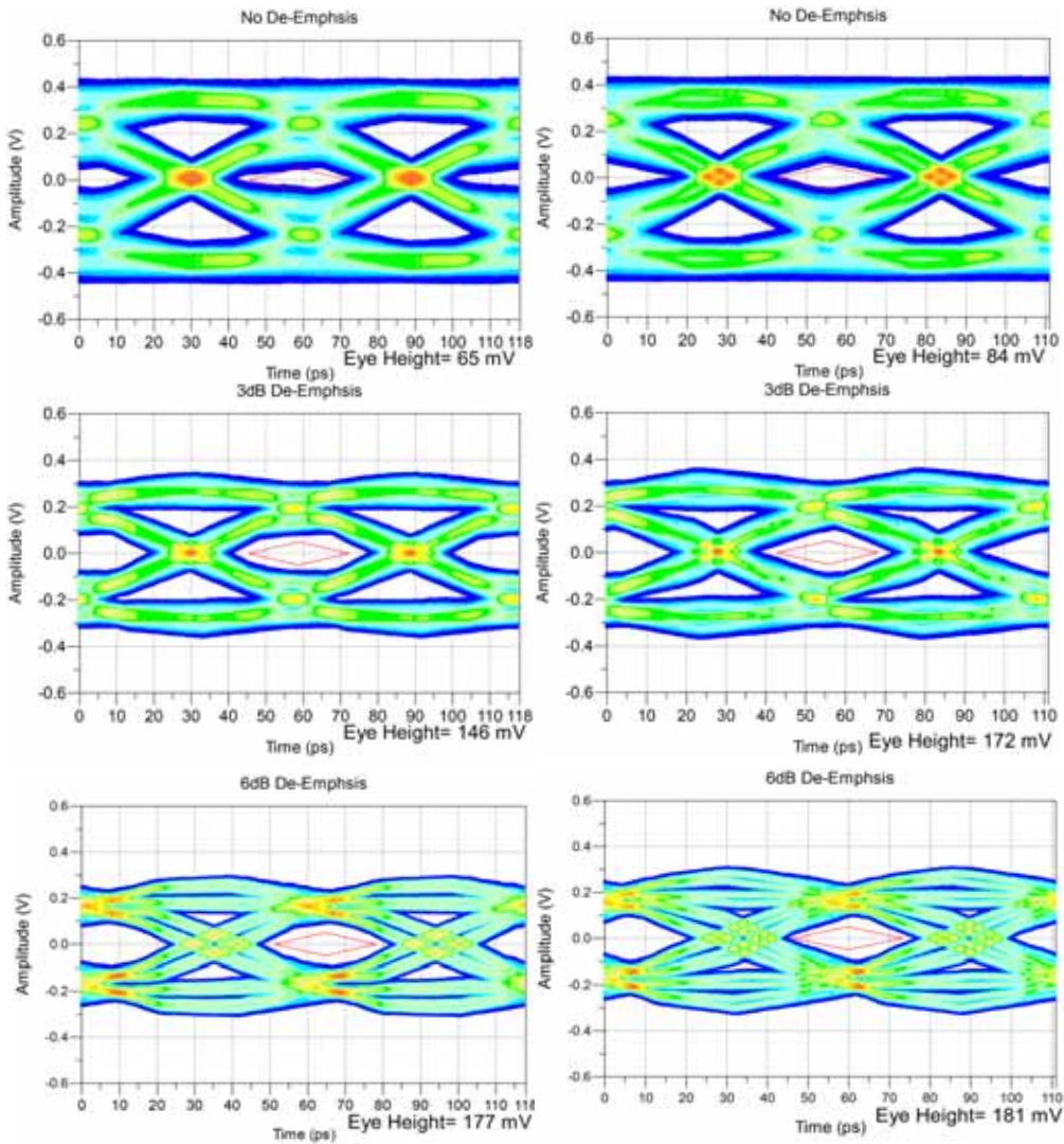
Long Row Output Eye : 17Gbps
