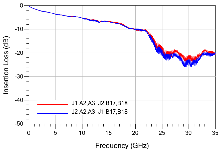
0.5m: Differential Application - Insertion Loss
