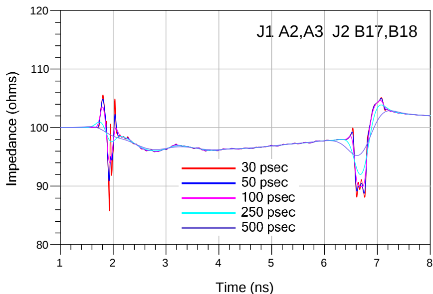
0.5m: Differential Application - Impedance
