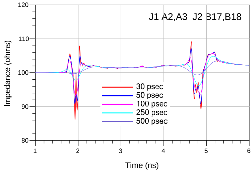
0.3m: Differential Application - Impedance
