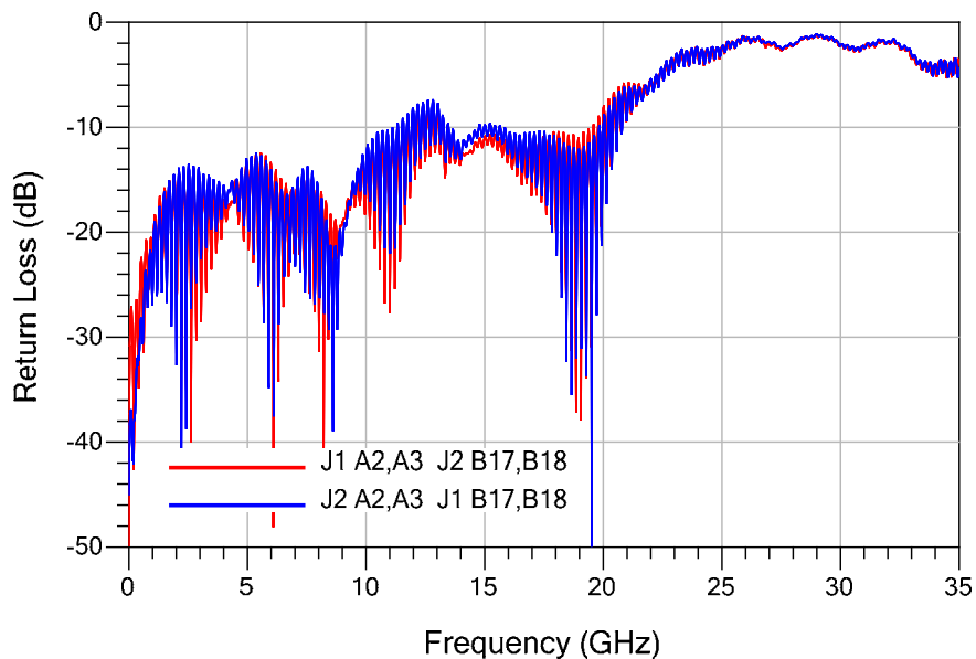
0.5m: Differential Application - Return Loss
