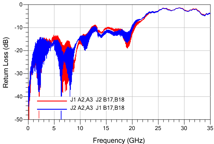
1m: Differential Application - Return Loss
