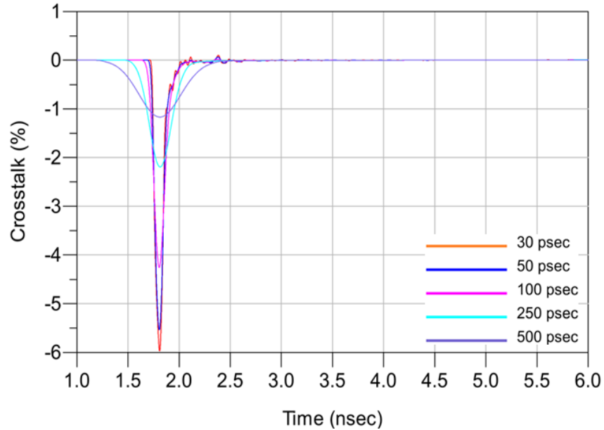
Differential Application - NEXT
