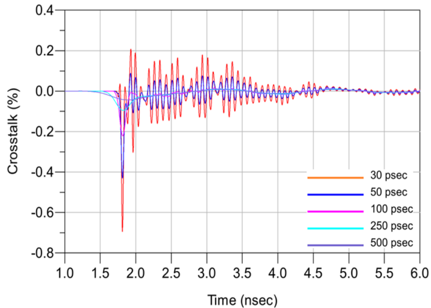
Single-Ended Application - FEXT
