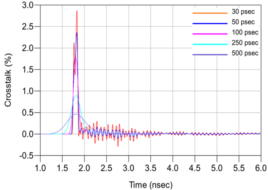
Single-Ended Application - NEXT
