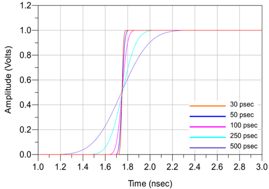
Single-Ended Application - Input Pulse
