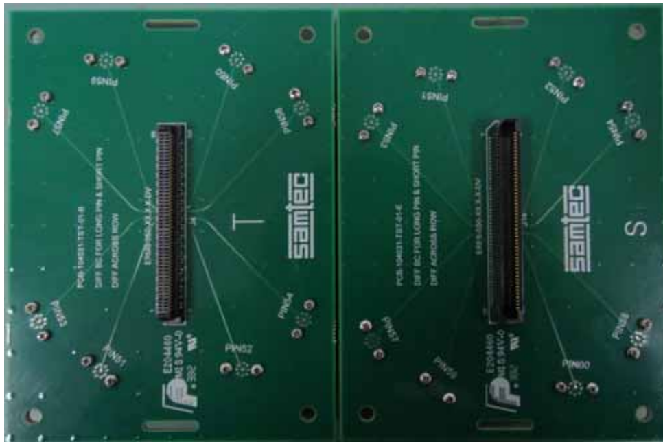
PCB-104031-TST-XX PCB Layout Panel
