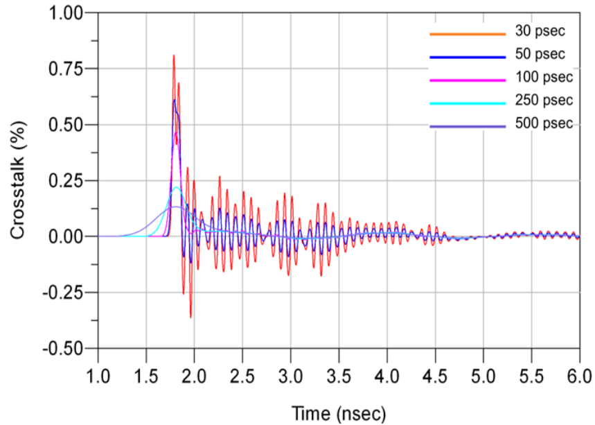
Single-Ended Application - NEXT
