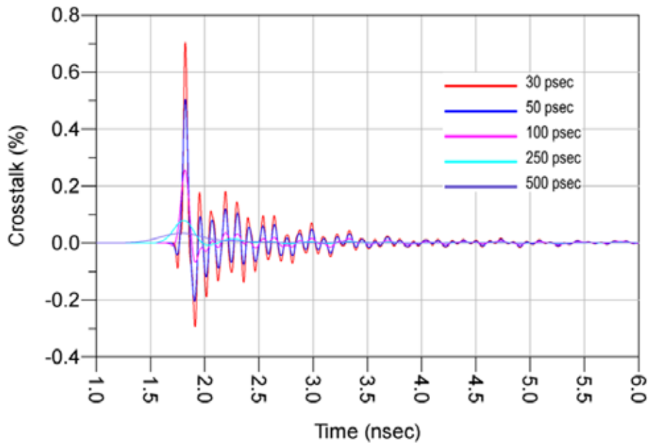
Differential Application - FEXT
