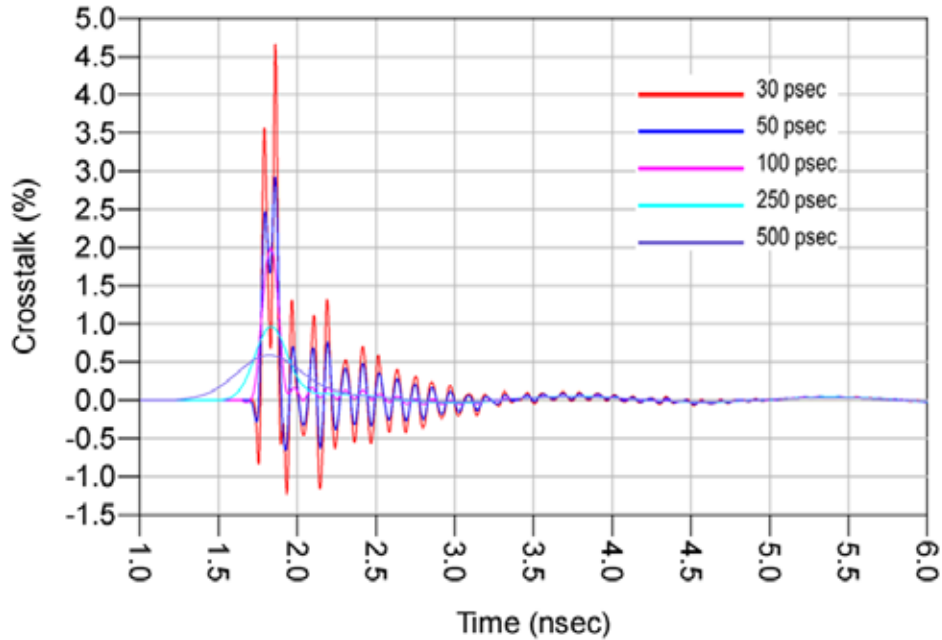
Single-Ended Application - NEXT
