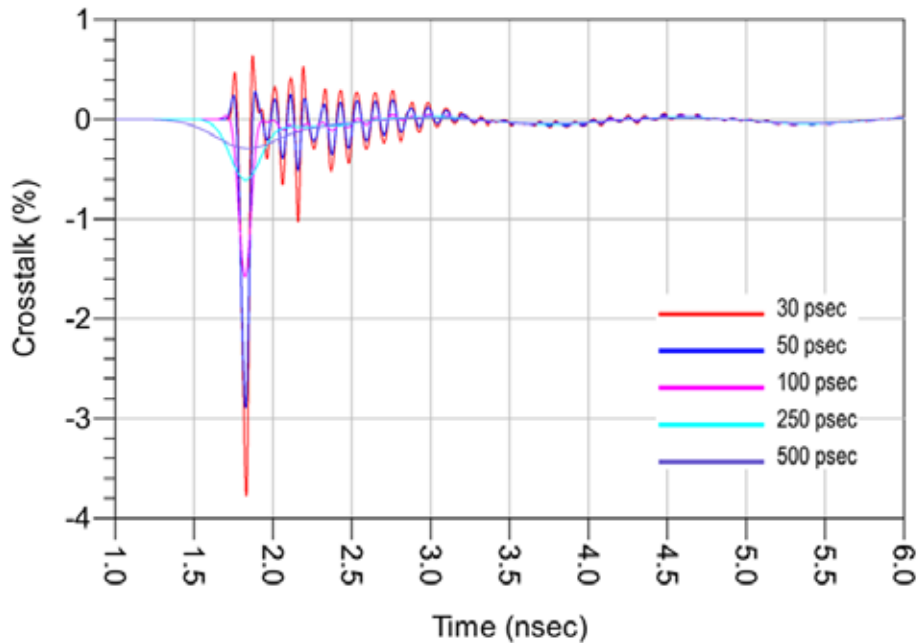
Single-Ended Application - FEXT
