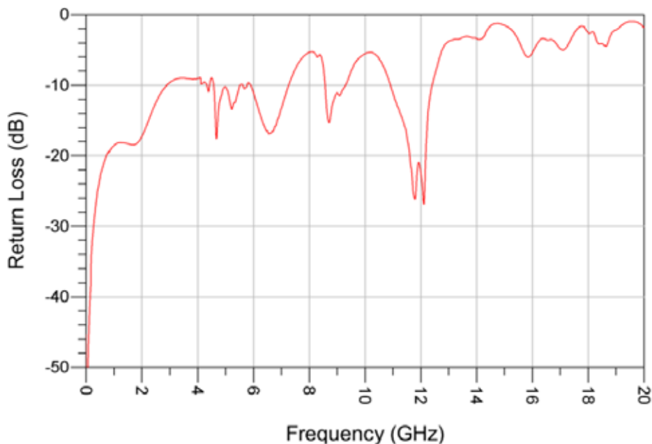
Single-Ended Application - Return Loss
