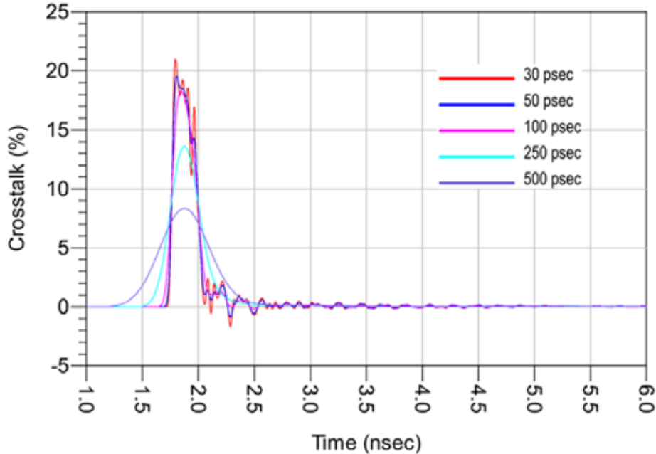
Single-Ended Application - NEXT
