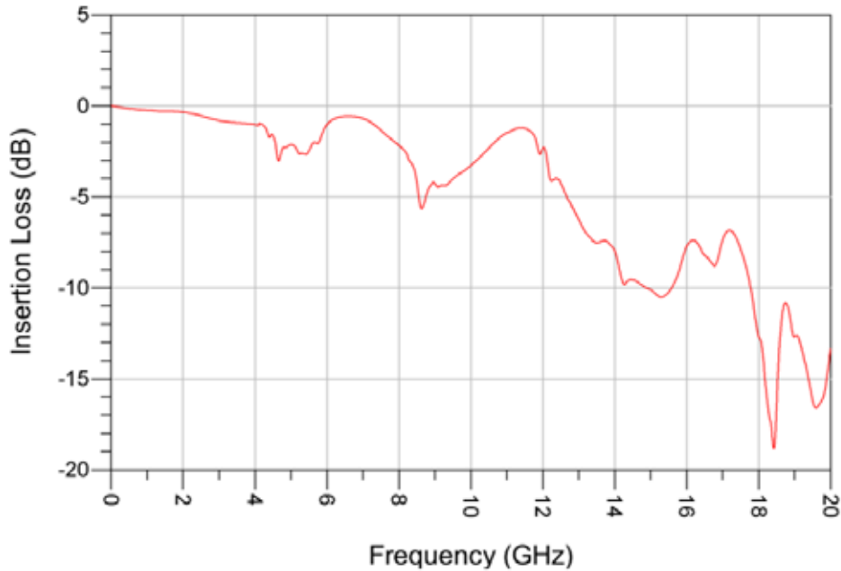
Single-Ended Application - Insertion Loss
