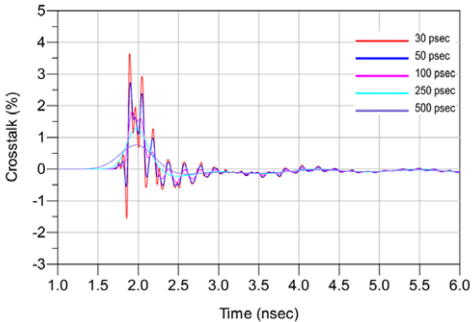
Single-Ended Application - FEXT
