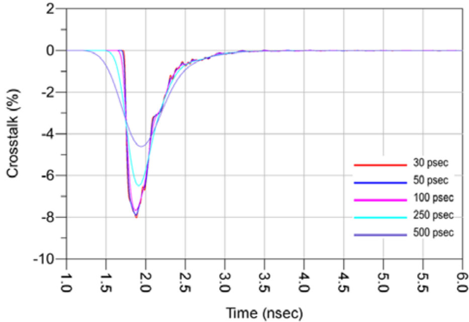
Differential Application - NEXT
