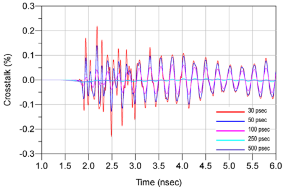
Single-Ended Application - FEXT
