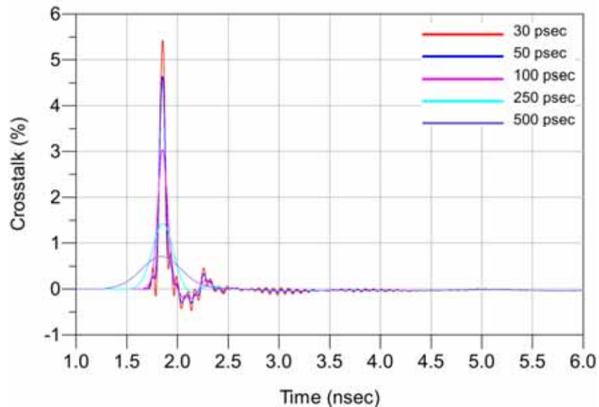
Single-Ended Application - FEXT
