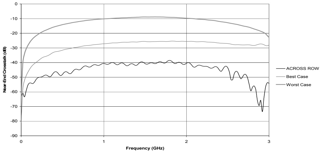
PCB/Connector Test System Single Ended Application BSE-01 / BTE-07
