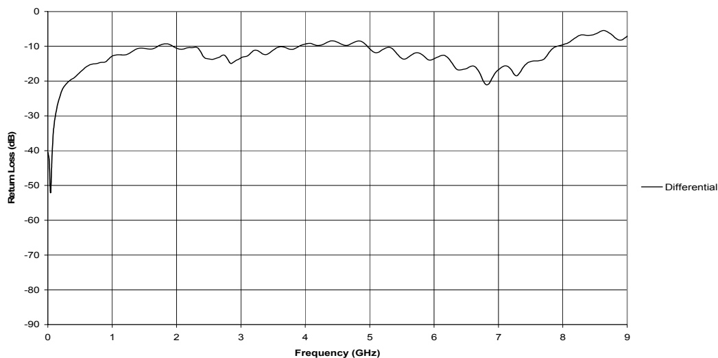
PCB/Connector Test System Differential Application MIS-01 / MIT-06 DP version
