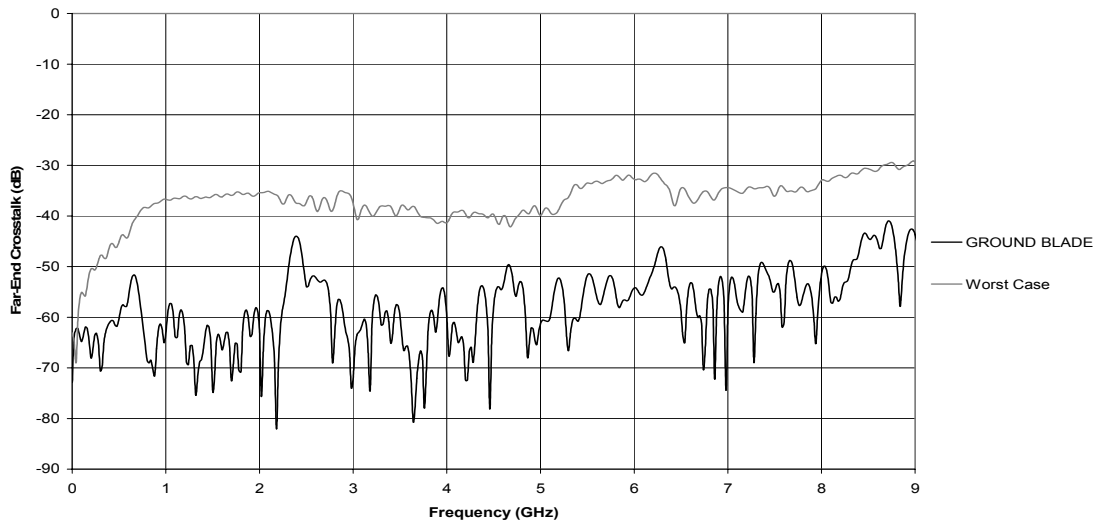
PCB/Connector Test System Differential Application MIS-01 / MIT-06 DP version
