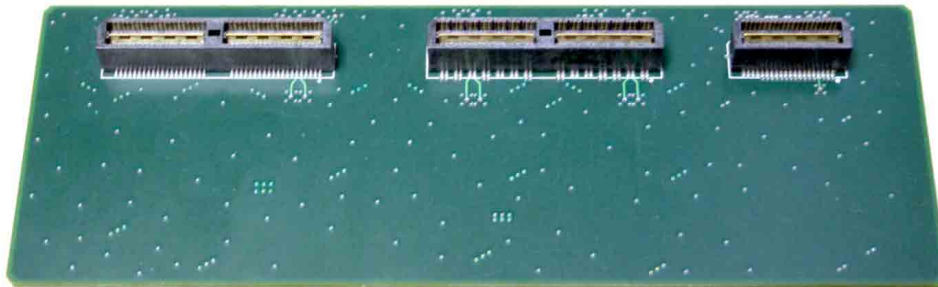
Figure 3 (Lt. to Rt.) QTE-040-01-X-D-A, QTE-028-01-X-D-A, QTE-020-01-X-D-A
