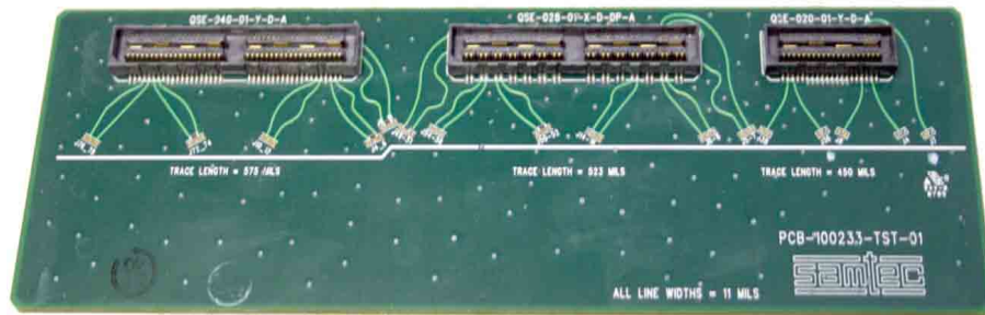
Figure 2 (Lt. to Rt.) QSE-040-01-X-D-A, QSE-028-01-X-D-A, QSE-020-01-X-D-A
