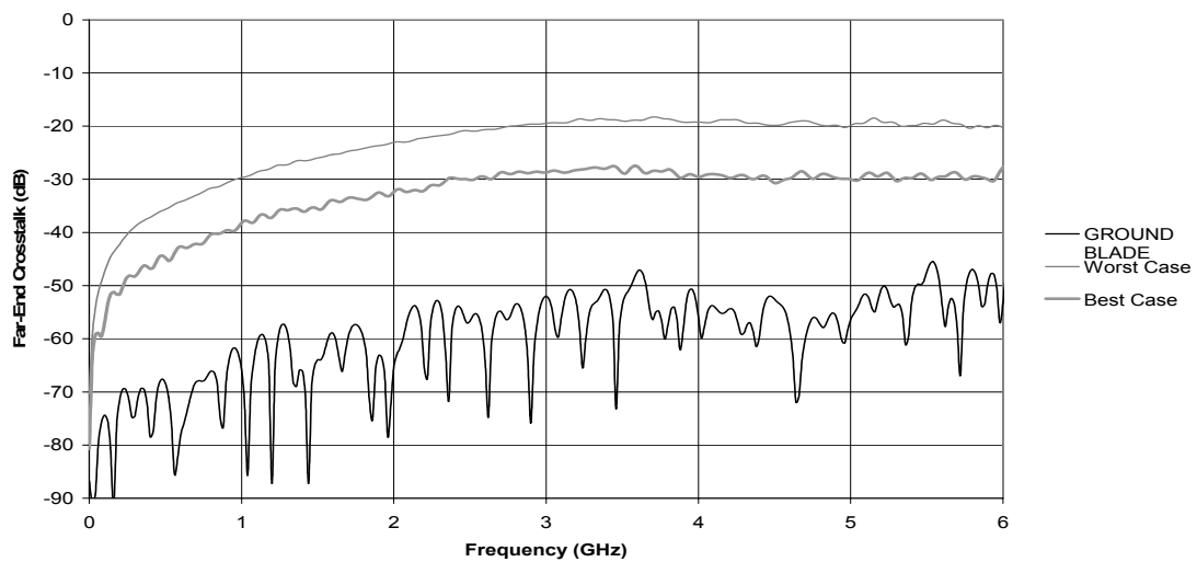
PCB/Connector Test System Single Ended Application QSE-01 / QTE-02 Series (8mm Stack Height)
