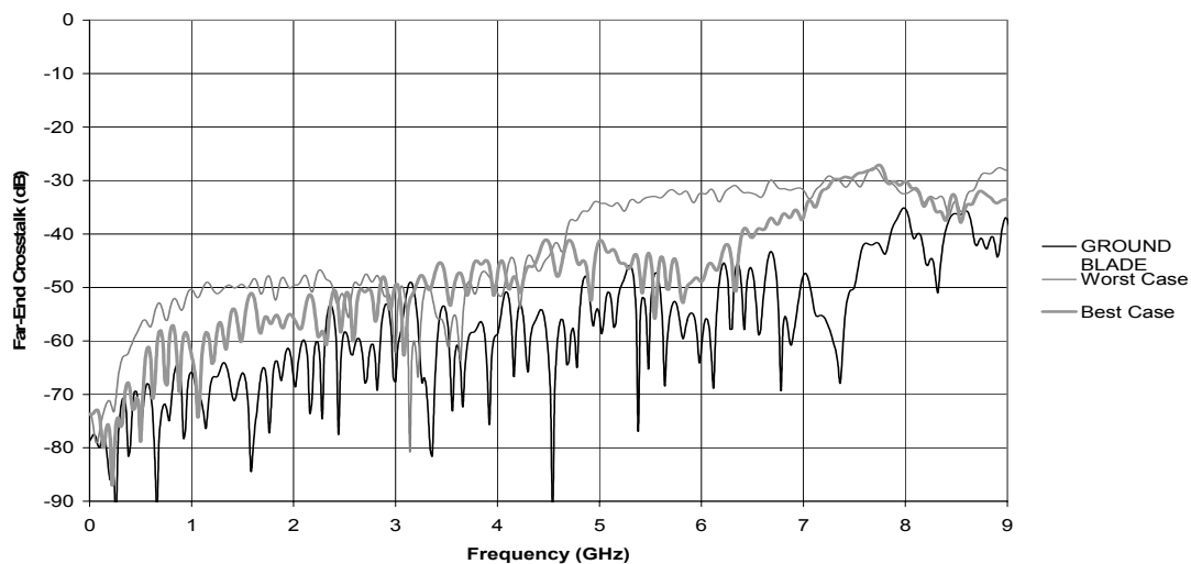
PCB/Connector Test System Differential Application QSE-01 / QTE-02 Series (8mm Stack Height)
