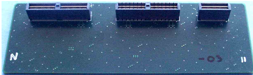
Figure 3 (Lt. to Rt.) QTE-040-03-X-D-A, QTE-028-03-X-D-A, QTE-020-03-X-D-A
