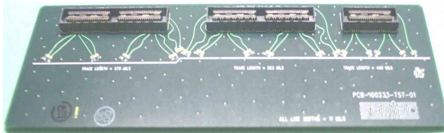
Figure 2 (Lt. to Rt.) QSE-040-01-X-D-A, QSE-028-01-X-D-A, QSE-020-01-X-D-A
