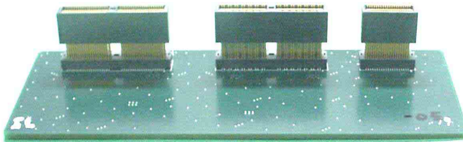
Figure 3 (Lt. to Rt.) QTE-040-05-X-D-A, QTE-028-05-X-D-A, QTE-020-05-X-D-A
