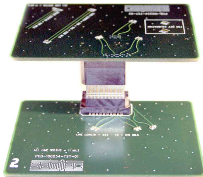
Figure 1 Mated PCB Test Fixture with Mounted Test Connectors
