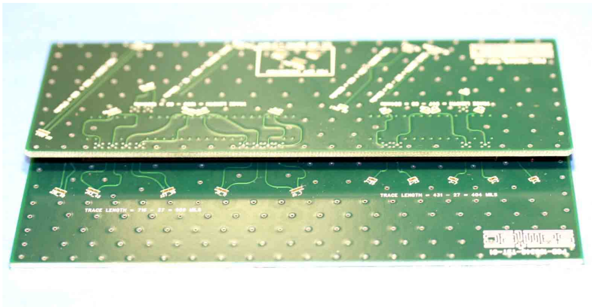
Figure 1 Mated PCB Test Fixture with Mounted Test Connectors
