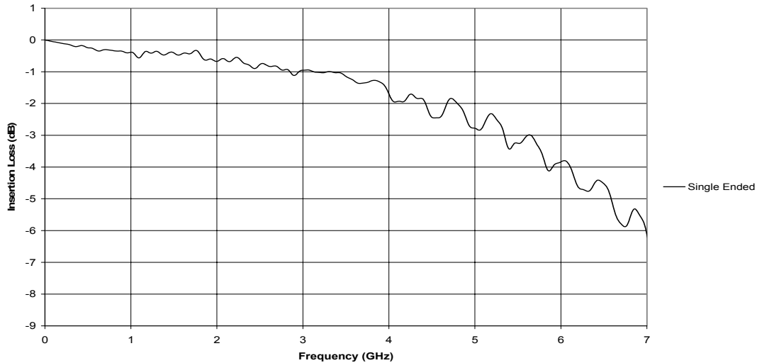
PCB/Connector Test System Single Ended Application CLT-02 / TMMH-05
