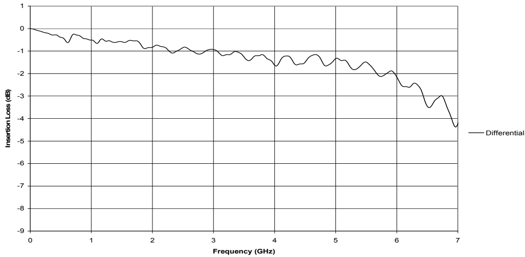
PCB/Connector Test System Differential Application CLT-02 / TMMH-05
