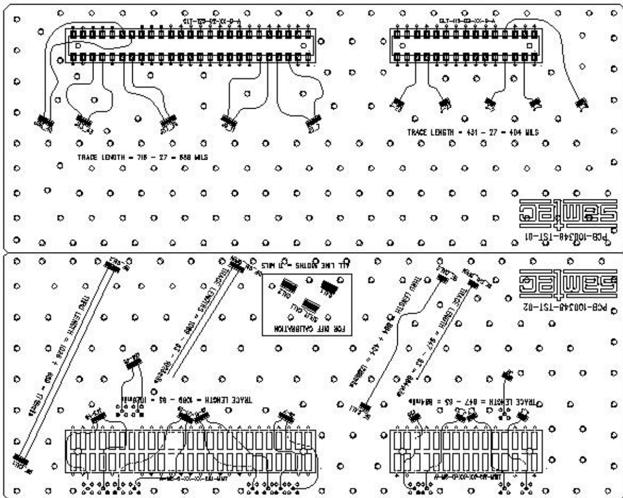
Figure 2 PCB Test Board Signal Routing
