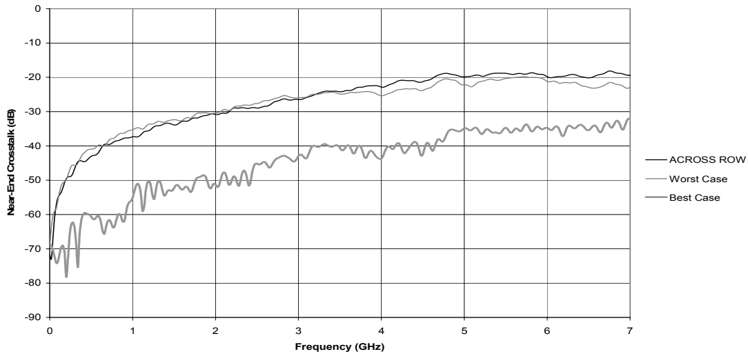
PCB/Connector Test System Differential Application CLT-02 / TMMH-05
