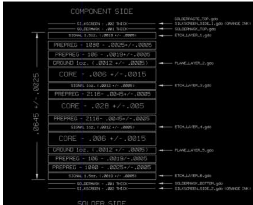
QTE/QSE Test board layer stackup
