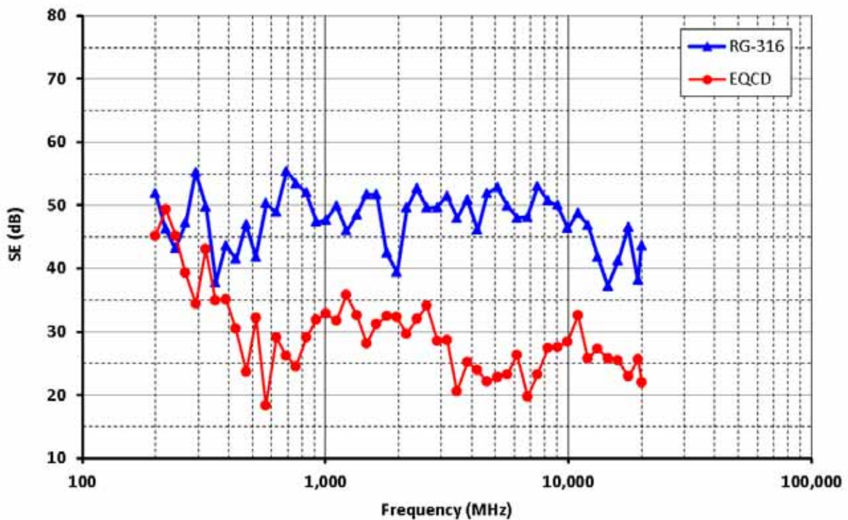
Shielding Effectiveness - EQCD and RG-316
