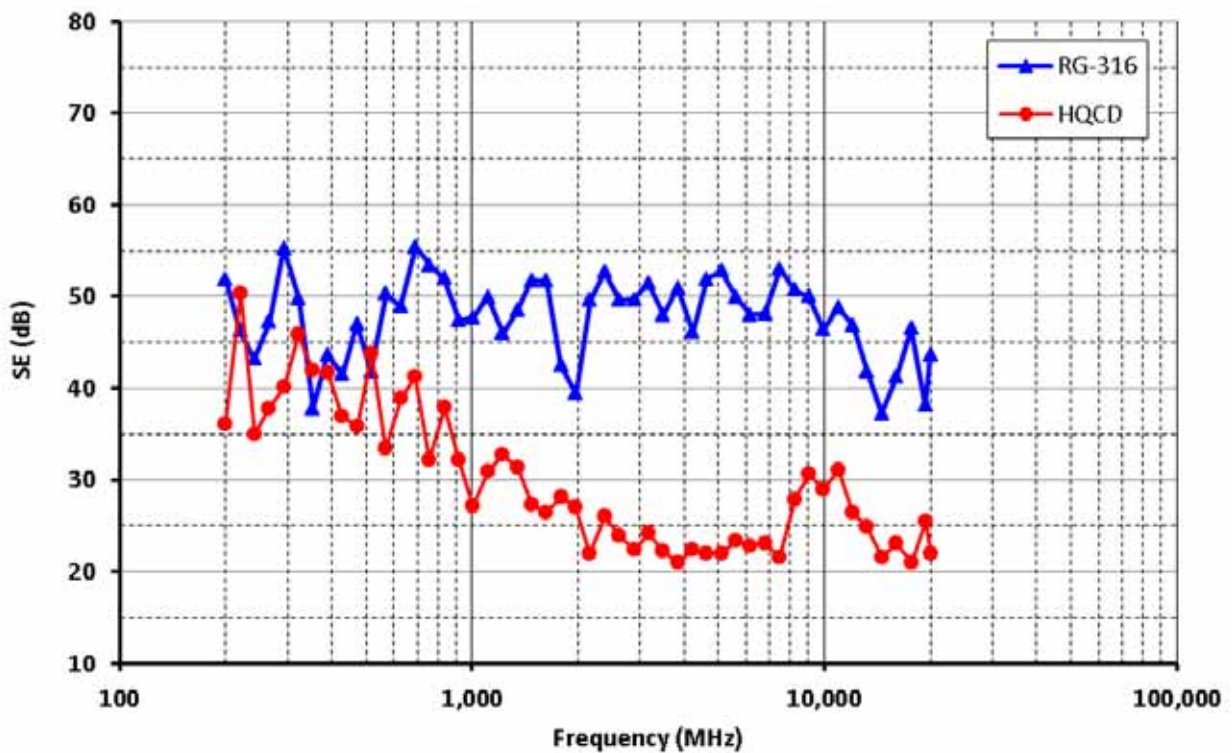
Shielding Effectiveness - HQCD and RG-316
