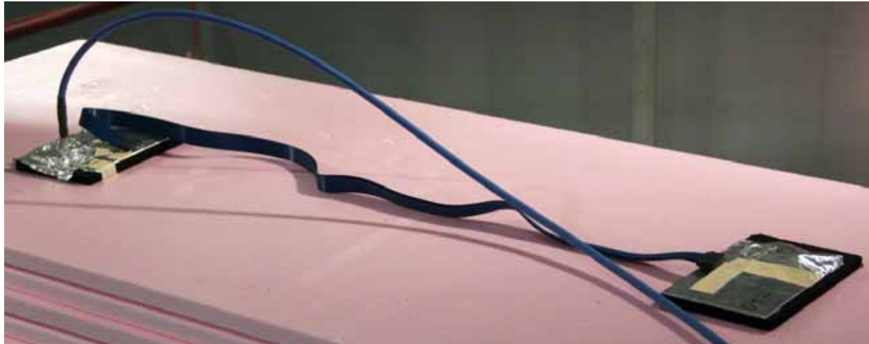
HQCD cable assembly in reverb chamber
